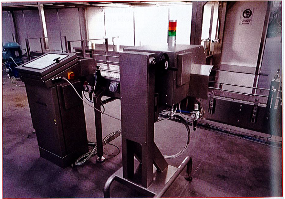
Above: ControlLevel XR x-ray technology, developed by Parmacontrols, checks fill levels and is particularly suitable for canning lines with rotary retorts
